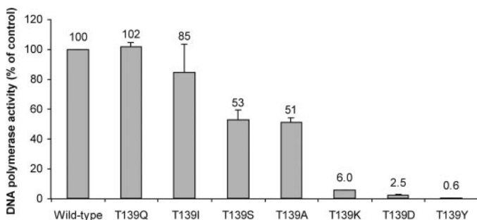
Fig. 2. Catalytic RNA-dependent DNA polymerase activity of mutant T139Q, T139I, T139S, T139A, T139K, T139D, and T139Y HIV-1 RT enzymes. 8 ng of wild type, 11 ng of T139A, 6 ng of T139Q, 61 ng of T139Y, 575 ng of T139K, 6 ng of T139I, 9 ng of T139S, and 137 ng of T139D mutant enzyme (protein) were used in the enzyme assays. Data ( \pm S.D.) are the means of at least two to three independent experiments.
